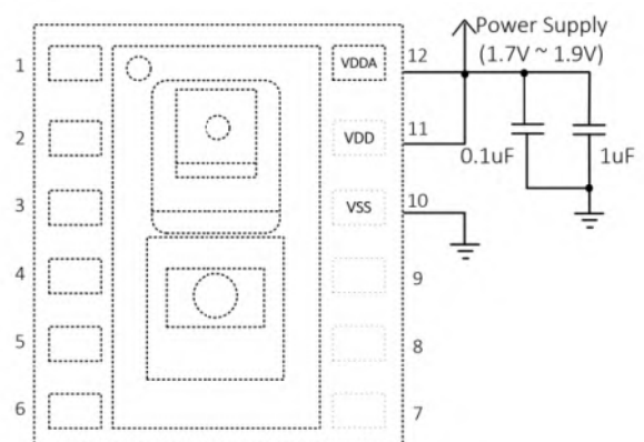
Figure 9. Low Voltage Segment
