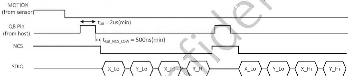
Figure 19. Quick Burst Function in SPI mode
